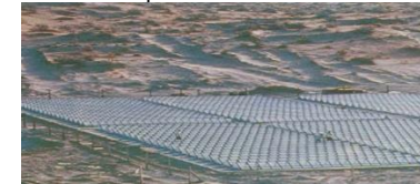
Solar desalter in the Central Kara Kum (Institute of solar energy at Academy of Science of Turkmenistan)
